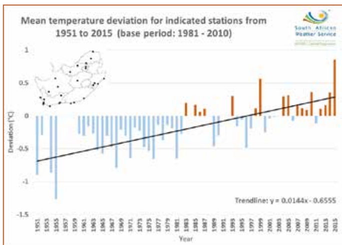
FIGURE 6: 1951 to 2015 annual mean near-surface temperature anomalies (°C), as calculated from the base period 1981–2010 and as recorded at 26 climate stations across South Africa (black dots on the map). The trend line indicates a warming of 0.14°C per decade. Source: South African Weather Service (SAWS) Department: Climate Service.
