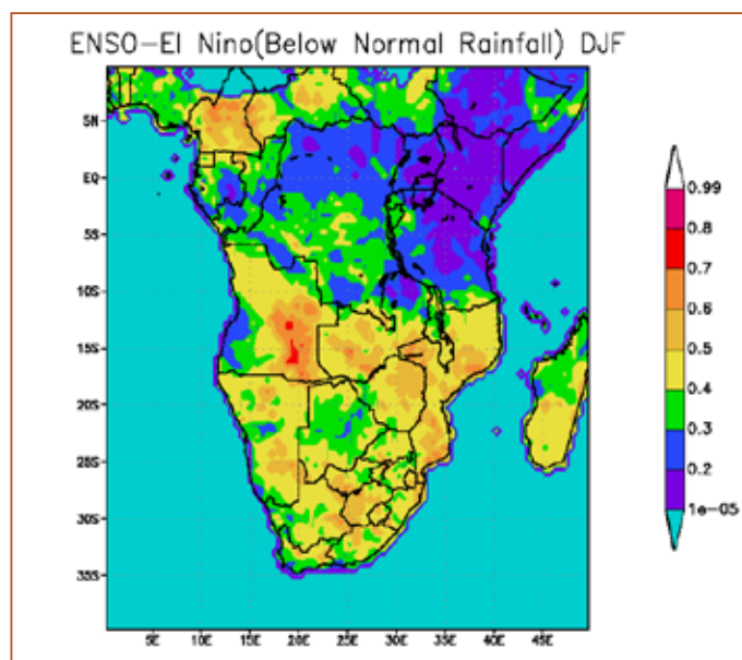
FIGURE 10: Between 50% and 60% of the time below-normal rainfall across southern Africa is associated with El Niño or positive ENSO events. Source: South African Weather Service (SAWS) Long-Range Forecasting Section.
