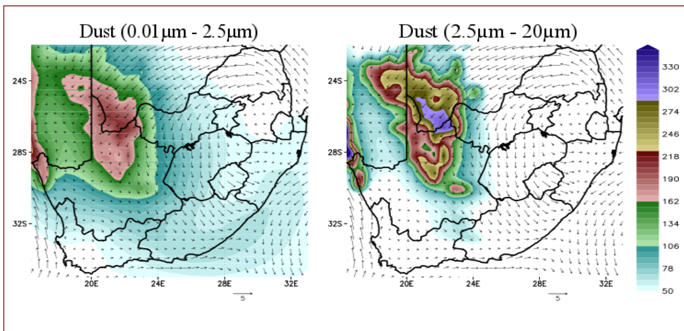
FIGURE 3: 12 years averaged (over 1998–2008) column load of wind eroded desert dust particles which are within the diameter range of 0.01 µm to 2.5 µm and 2.5 µm to 20 µm (shaded, unit: mg/m 2 ), superposed with the 10 m wind field (vector; the scale is indicated by the arrow to the lower right; unit: m/s), in and around South Africa.. This figure is generated based on Tesfaye et al. 2015 – interactively coupled model simulation results which were published in Journal of Arid Environments .
