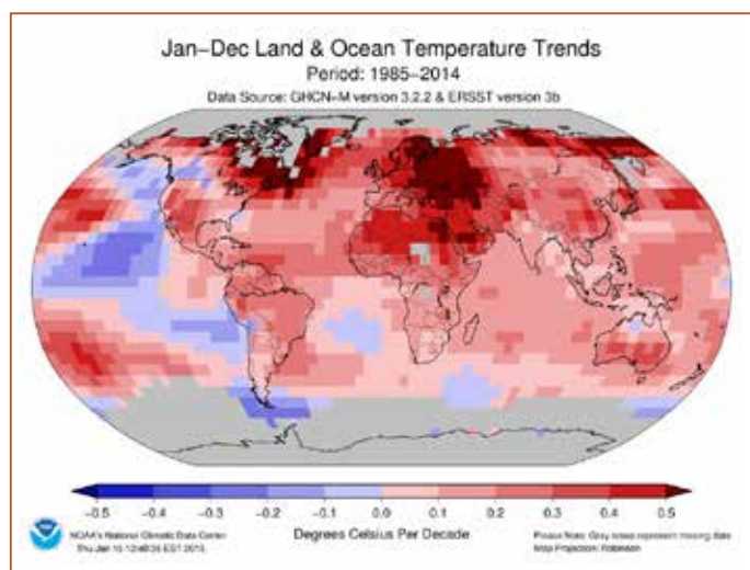
FIGURE 7: 1985 to 2014 global near-surface temperature trends (°C per decade). Source: NOAA's National Climate Data Centre.
