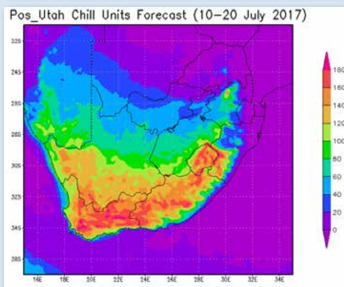
Figure 5: Chill units forecast calculated using the Positive Chill Units Model (chill units) with data from the ECMWF model 10 day forecast accumulated for the period of 10 to 19 July 2017
