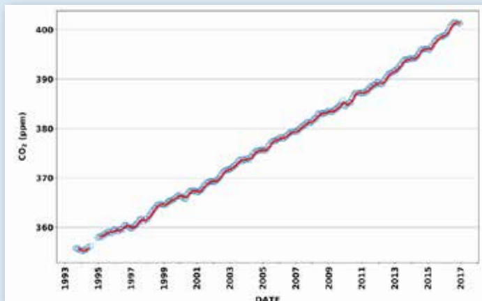
Figure 2: Cape Point \text{CO}_2 time series (1993-2017) showing monthly means, moving average (red)
