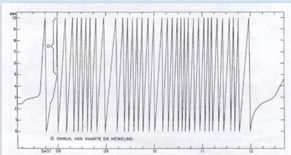
Figure 2: Reproduction of 1 September 1968 Rainfall chart (Port Elizabeth Airport)
