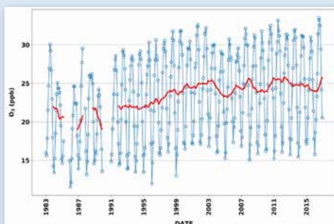
Figure 5: \text{O}_3 time series of monthly means (1983-2017) and moving average (red)
