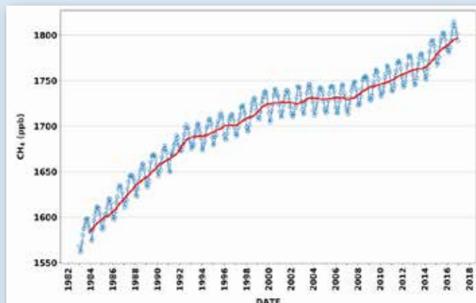
Figure 3: Cape Point \text{CH}_4 monthly means (1983-2017) for BG data where the red line highlights the moving average and a strong seasonal cycle is observed
