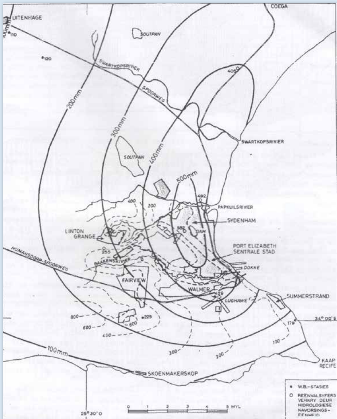
Figure 4: Isohyet for Port Elizabeth 1 September 1968. Dotted lines are contours
