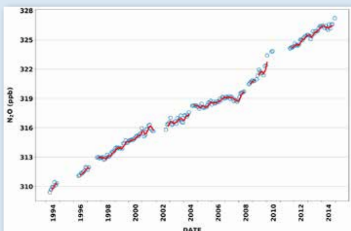
Figure 4: Monthly means of \text{N}_2\text{O} at Cape Point from 1993 till December 2015
