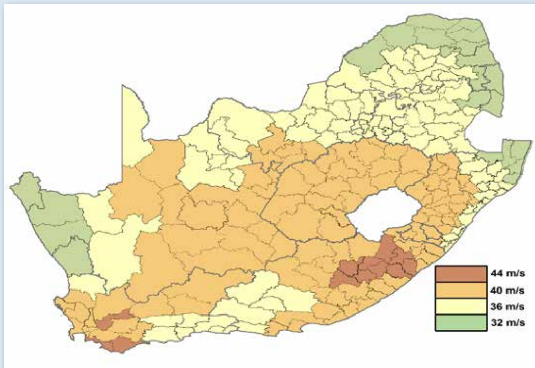
Figure 5: Map of the fundamental wind speed assigned to local municipal level, as presented by Kruger, Goliger and Retief in the Journal of the South African Institution of Civil Engineering (December 2017 issue)
