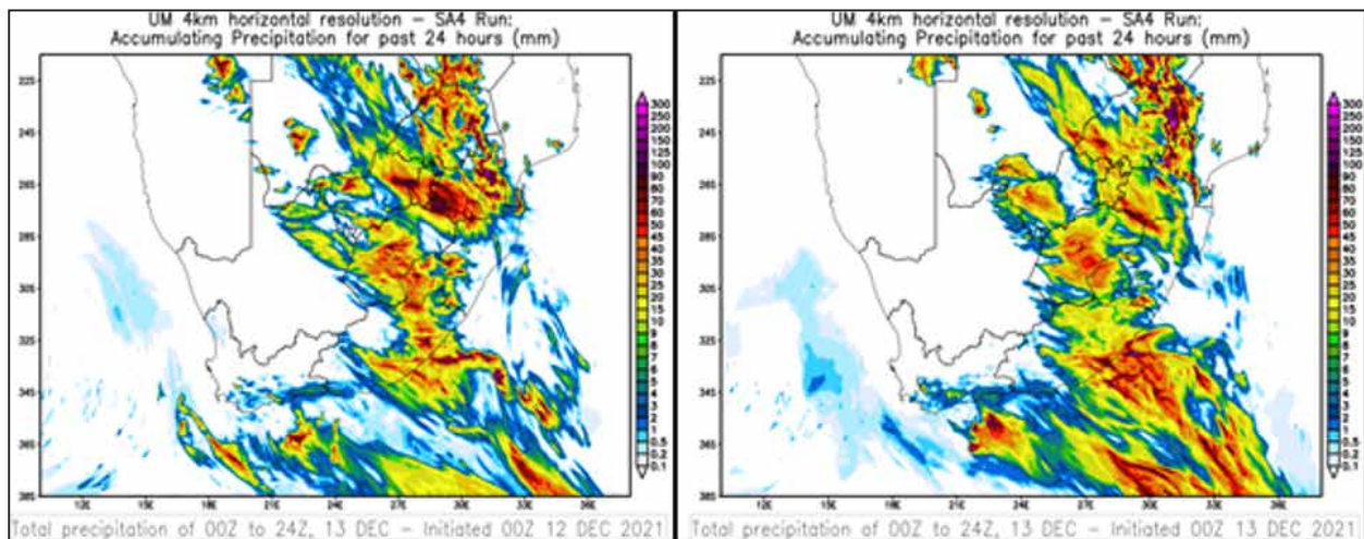
Figure 12: Image indicating total expected precipitation for 13 December 2021 using the UM4km 00Z for 12 and 13 December, with high values indicated between Fort Beaufort and Coffee Bay
