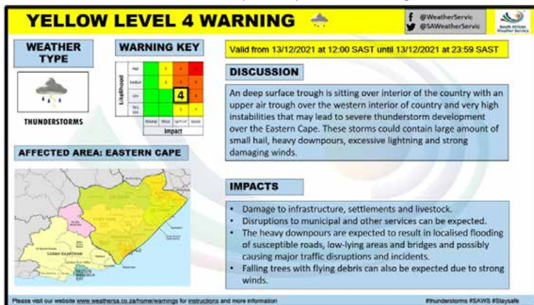
Figure 14: IBF warning issued for the eastern half of the Eastern Cape on 13 December 2021
