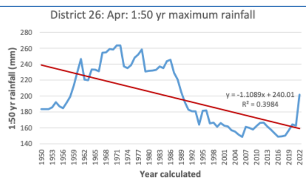
Figure 6: April 1:10 year (left) and 1:50 year (right) maximum rainfall (mm) for District 26, based on the 30-year periods ending in the years as indicated on the x-axis. The red line presents the linear trend.
