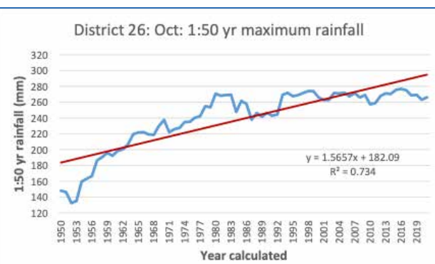
Figure 5: October 1:10 year (left) and 1:50 year (right) maximum rainfall (mm) for District 26, based on the 30-year periods ending in the years as indicated on the x-axis. The red line presents the linear trend.
