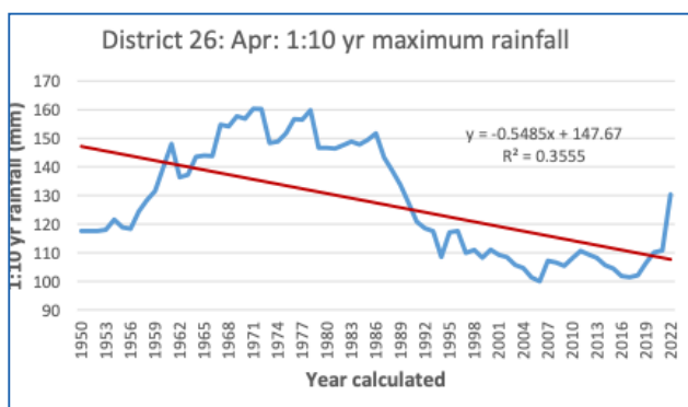
Figure 6: April 1:10 year (left) and 1:50 year (right) maximum rainfall (mm) for District 26, based on the 30-year periods ending in the years as indicated on the x-axis. The red line presents the linear trend.
