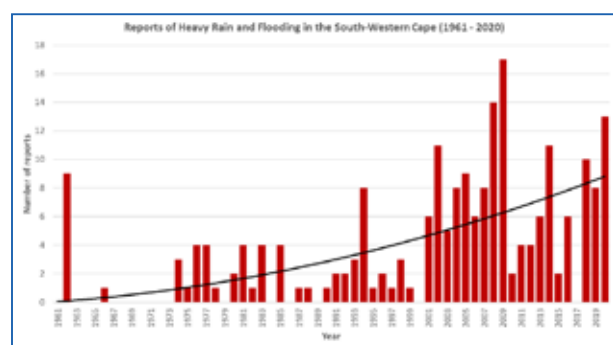
Figure 11: Annual number of reports on heavy rain and flooding in the South-Western Cape over the period 1961 – 2020.
