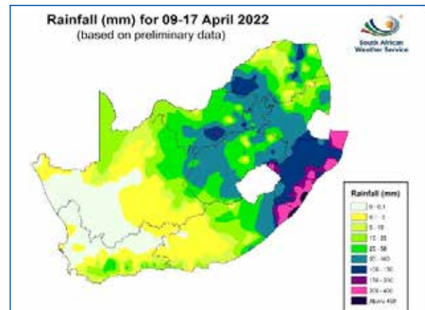
Figure 4: Accumulated rainfall received over period 9 to 17 April 2022
