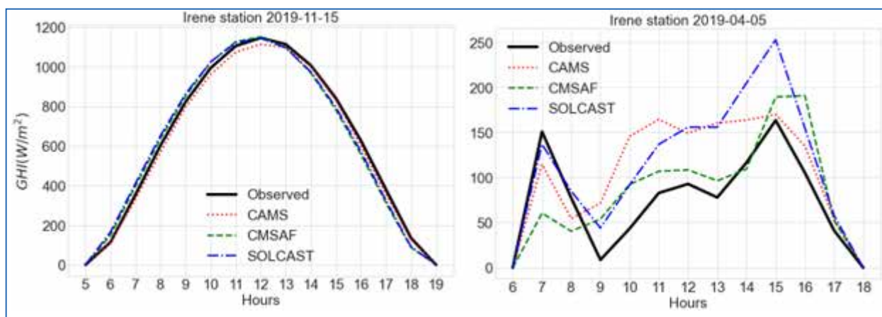
Figure 2: (a, left) Hourly clear-sky day and (b, right) overcast-sky day {Cloud cover information was detected by using CLAAS-2 satellite-based dataset}
