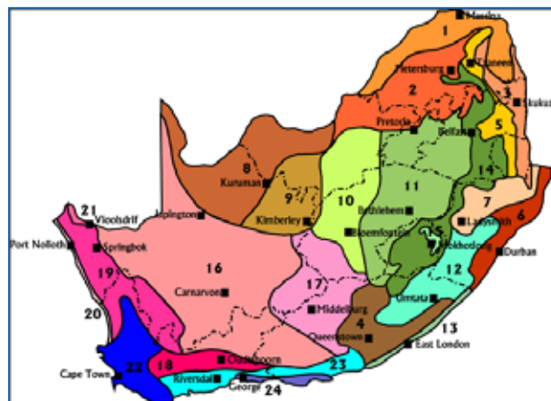
Figure 2: The Climatic Regions of South Africa: 1. Northern Arid Bushveld 2. Central Bushveld 3. Lowveld Bushveld 4. South-Eastern Thornveld 5. Lowveld Mountain Bushveld 6. Eastern Coastal Bushveld 7. KwaZulu-Natal Central Bushveld 8. Kalahari Bushveld 9. Kalahari Hardveld Bushveld 10. Dry Highveld Grassland 11. Moist Highveld Grassland 12. Eastern Grassland 13. South-Eastern Coast Grassland 14. Eastern Mountain Grassland 15. Alpine Heathland 16. Great and Upper Karoo 17. Eastern Karoo 18. Little Karoo 19. Western Karoo 20. West Coast 21. North-Western Desert 22. Southern Cape Forest 23. South-Western Cape 24. Southern Cape.
