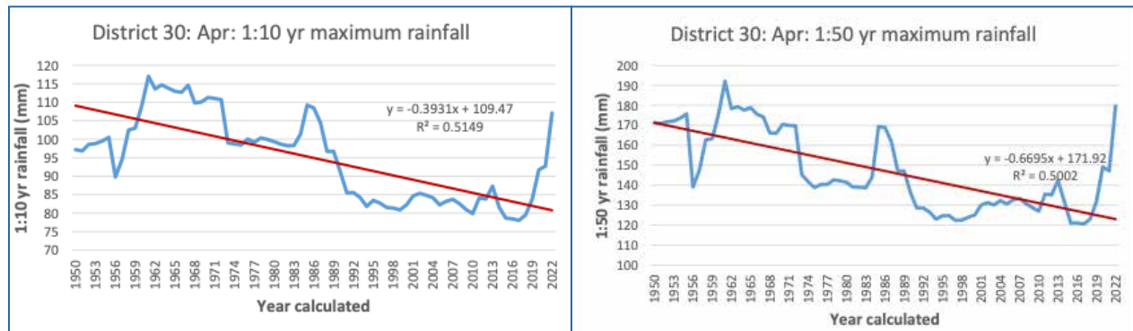
Figure 7: April 1:10 year (left) and 1:50 year (right) maximum rainfall (mm) for District 30, based on the 30-year periods ending in the years as indicated on the x-axis. The red line presents the linear trend.
