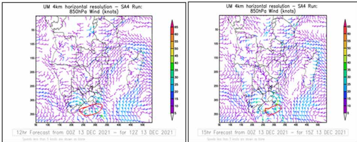
Figure 11: Images showing 850hPa winds at 12Z and 15Z, with the convergence over the western parts of the province at 12Z, moving the eastern parts at 15Z
