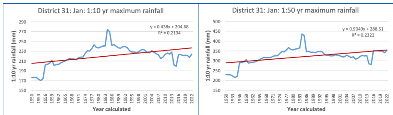
Figure 8: January 1:10 year (left) and 1:50 year (right) maximum rainfall (mm) for District 31, based on the 30-year periods ending in the years as indicated on the x-axis. The red line presents the linear trend.
