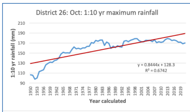
Figure 5: October 1:10 year (left) and 1:50 year (right) maximum rainfall (mm) for District 26, based on the 30-year periods ending in the years as indicated on the x-axis. The red line presents the linear trend.
