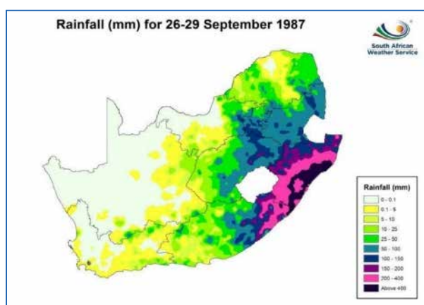
Figure 3: Accumulated rainfall received over period 26 to 29 September 1987
